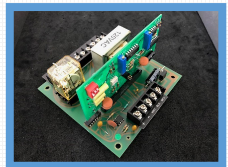
PN 1726 A1000 Circuit Board Assembly (PN1315, PN1325, PN1320)
